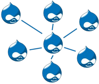
Drupal 7 Multi-site
